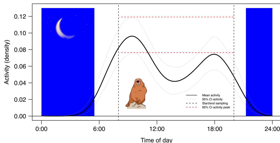
Figure 2. Kernel density estimate (with bootstrap 95% CI for the 95th percentile) of daily activity cycle of marmots in the study area in June 2019. Vertical dashed black lines indicate the timeframe (08:00–20:00 h) used for estimating availability and collecting data with distance sampling and CMR methods; horizontal dashed red lines indicate the estimated uncertainty of activity peak. Blue bars represent night hours.
